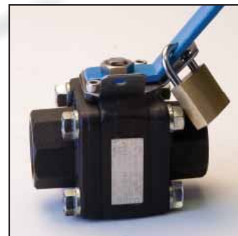
Integral Locking Device Padlock shown for illustration only. Customer to supply own lock.
