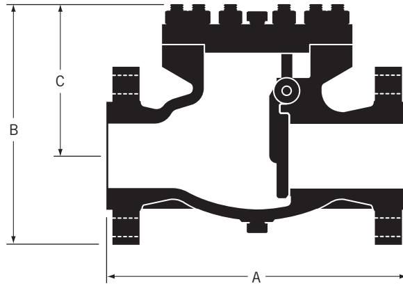
Dimensional Data • Class 150-1500, 2"- 6", (in.)
